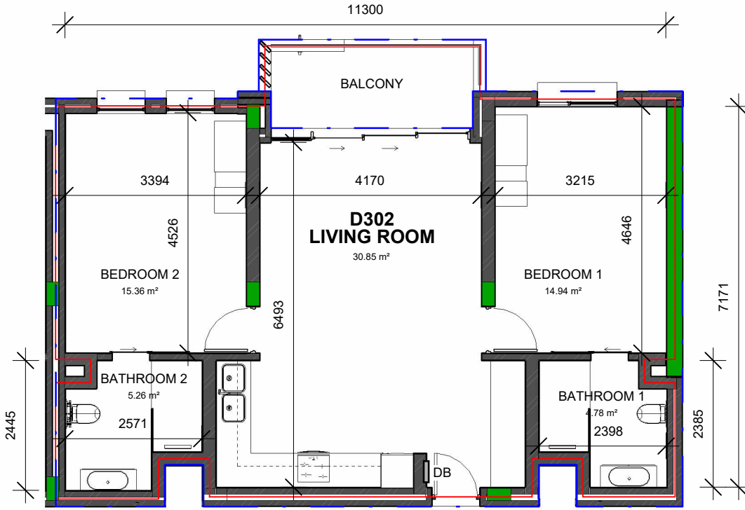
1:100 FLOOR PLAN
