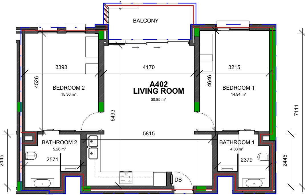
1:100 FLOOR PLAN
