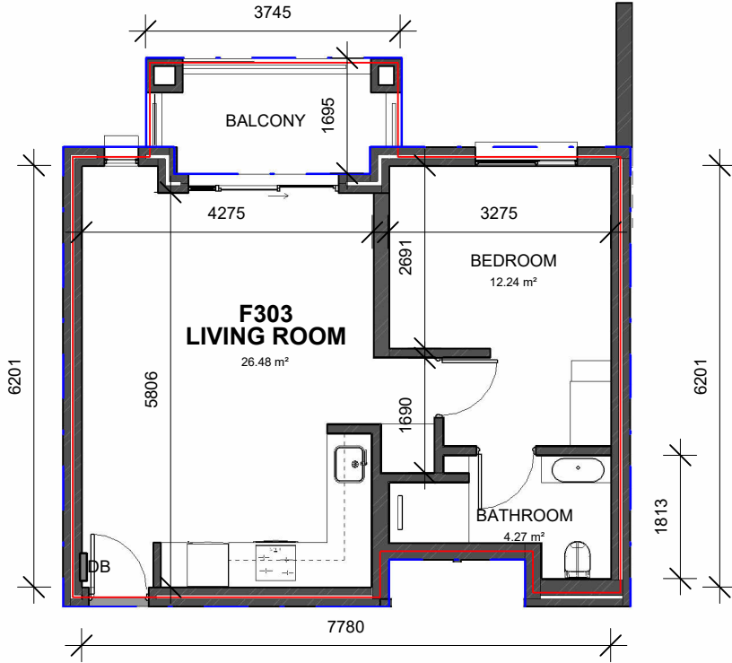
1:100 FLOOR PLAN
