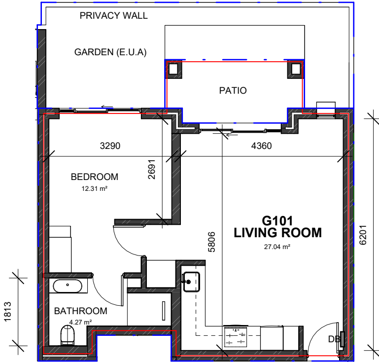
1:100 FLOOR PLAN
