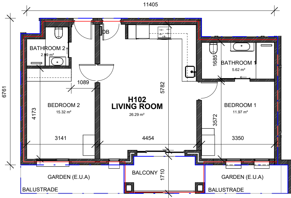
1:100 FLOOR PLAN
