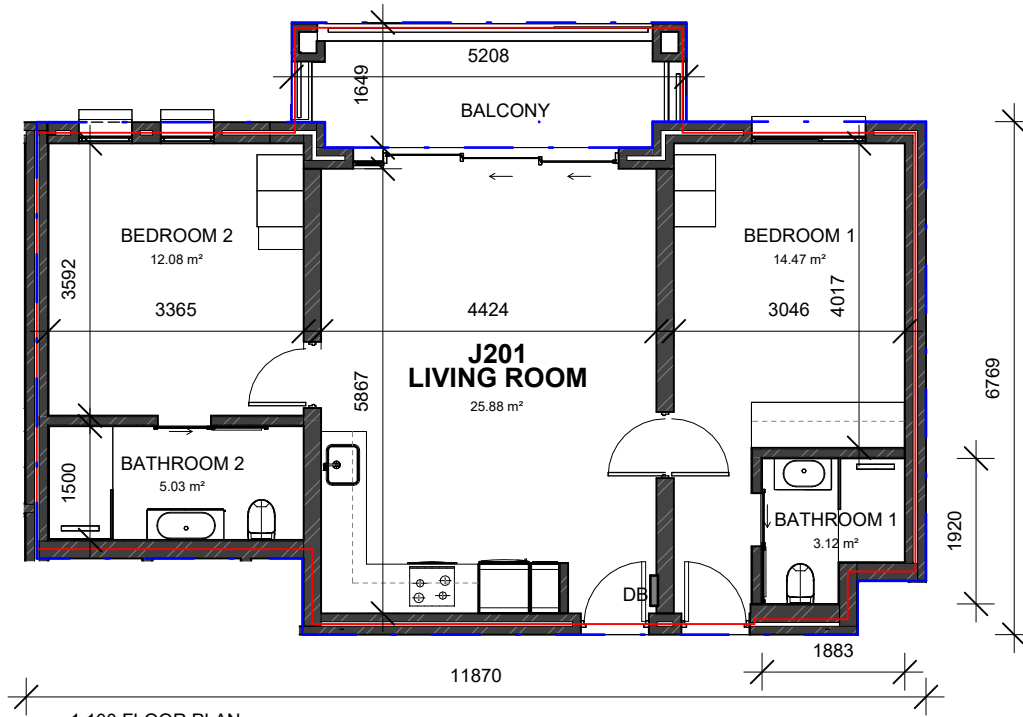
1:100 FLOOR PLAN
