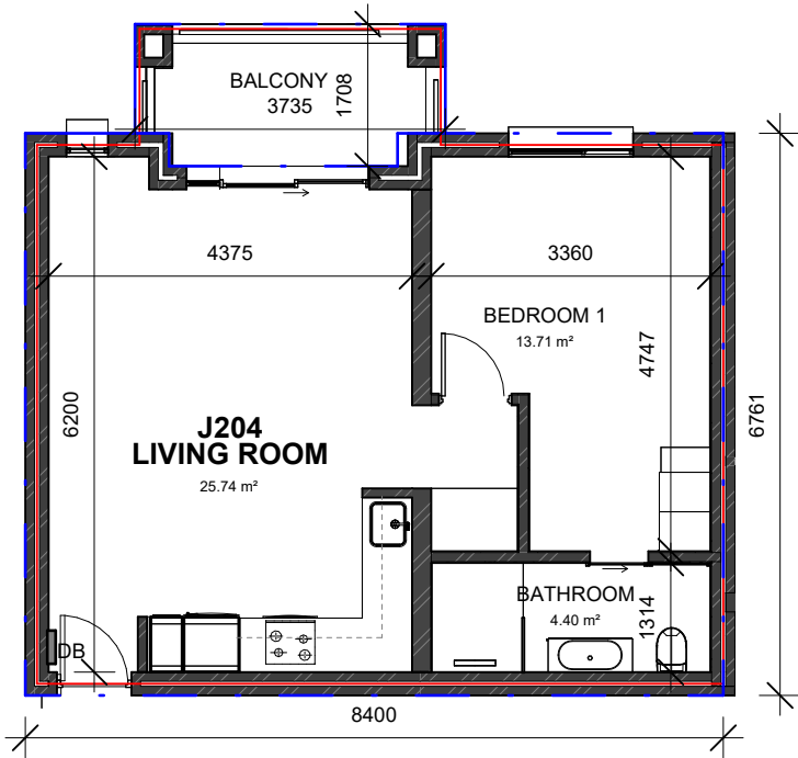
1:100 FLOOR PLAN
