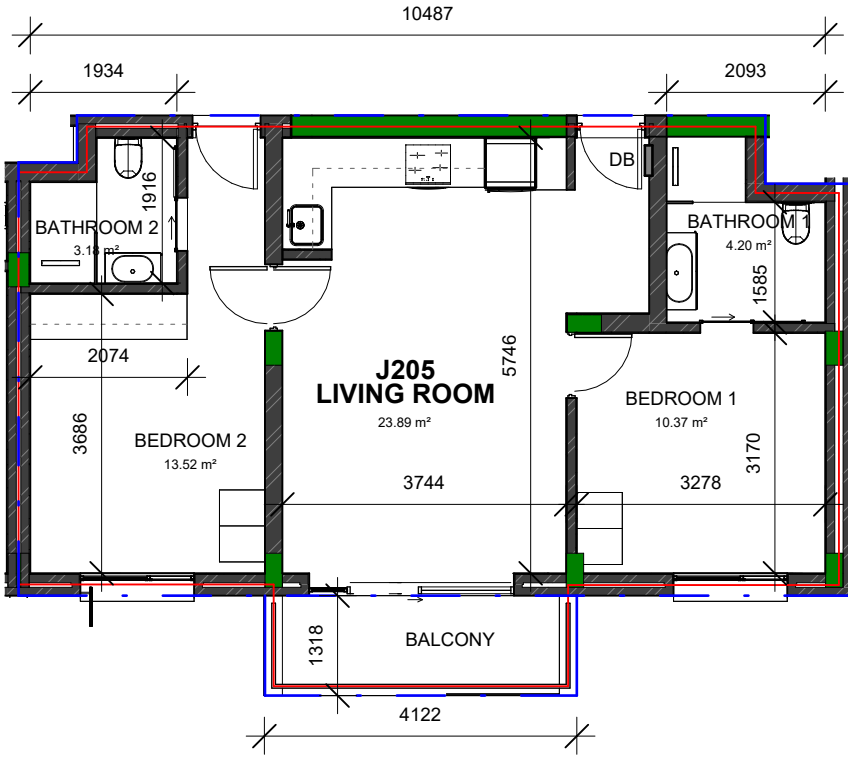
1:100 FLOOR PLAN
