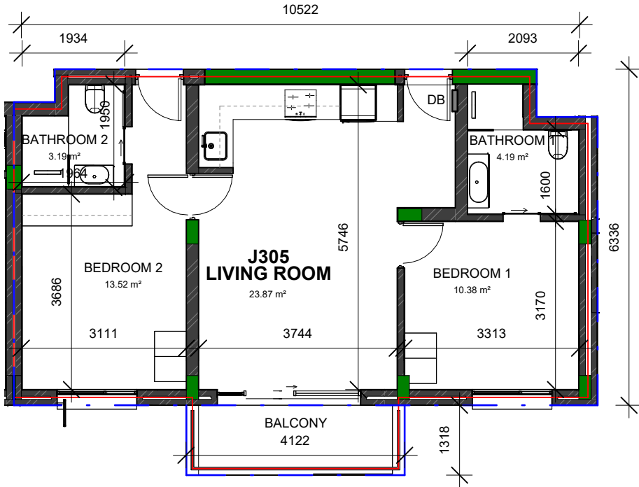
1:100 FLOOR PLAN
